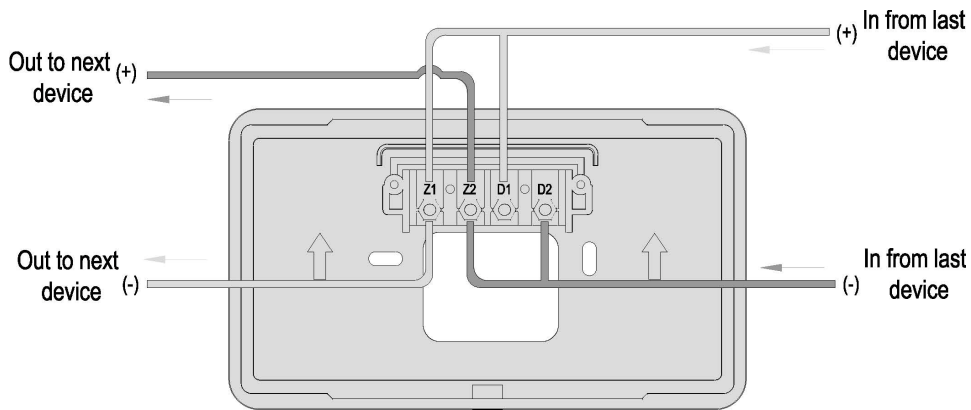
Figure 4 Loop Powered
